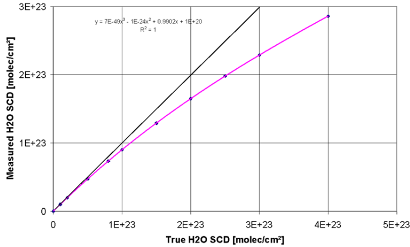
Figure 14 Relation between "true" H 2 O slant column from a line-by-line modelling, and the "measured" H 2 O slant column derived from a fit of the DOAS cross sections to the GOME-convolved absorption spectrum. Dots represent the calculations; the pink line is the polynomial fit from Eq. (27) - the black line indicates equality.
