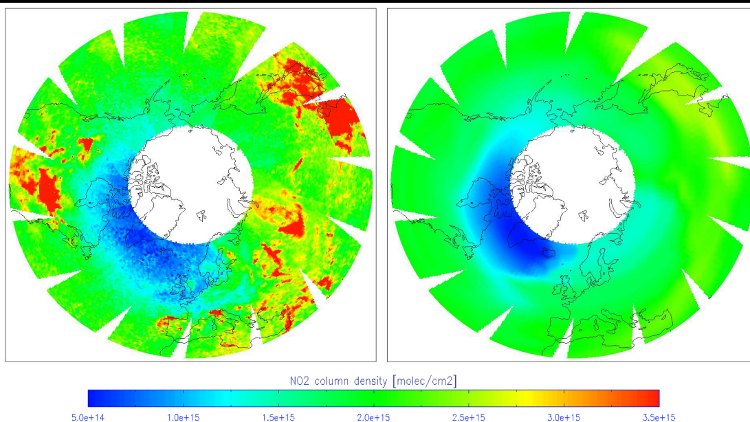
Figure 9 Total NO 2 distribution from GOME-2/MetOp-A for 22 February 2008 (left) and the corresponding stratospheric NO 2 distribution as obtained with the spatial filtering approach (right).
