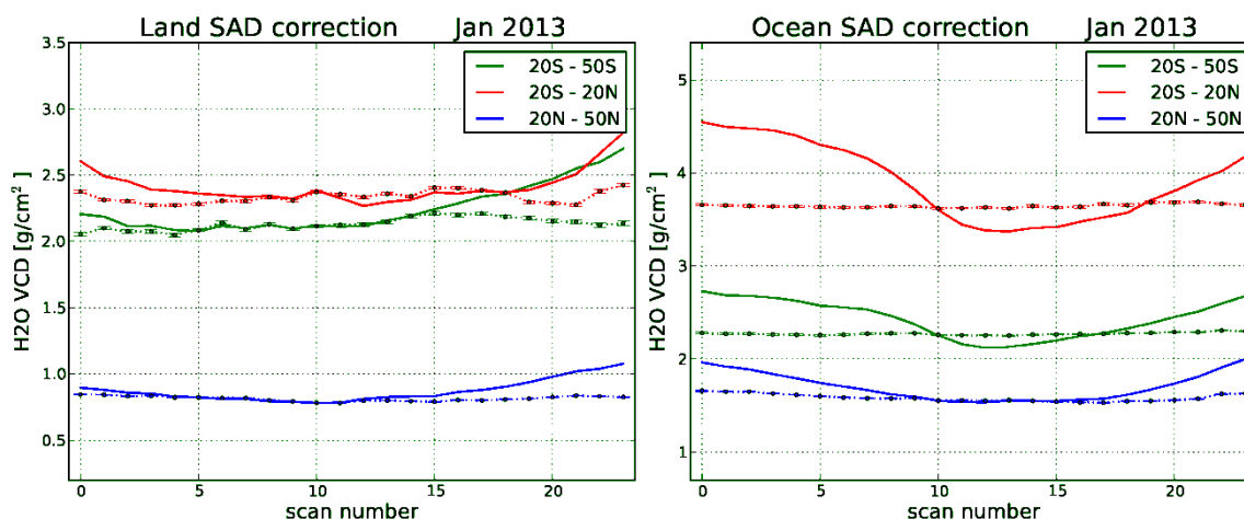
Figure 18 GOME-2A H 2 O VCD as a function of pixel index within the scan (0=East, 24=West) averaged in different latitude bands (20°S - 50°S, 20°S - 20°N, 20°N - 50°N) before (solid line) and after (dashed line with points) the scan angle dependency correction for January 2013. We show separately the empirical correction applied over land measurements (left panel) and over ocean measurements (right panel).
