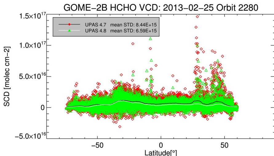
Figure 11 Single orbit of GOME-2B showing the reduced scatter in GDP v4.8/4.9 compared to GDP 4.7 due to implementation of a second fitting window for BrO. Plotted are the individual measurements and its averages (lines) within 5° latitude bands.
