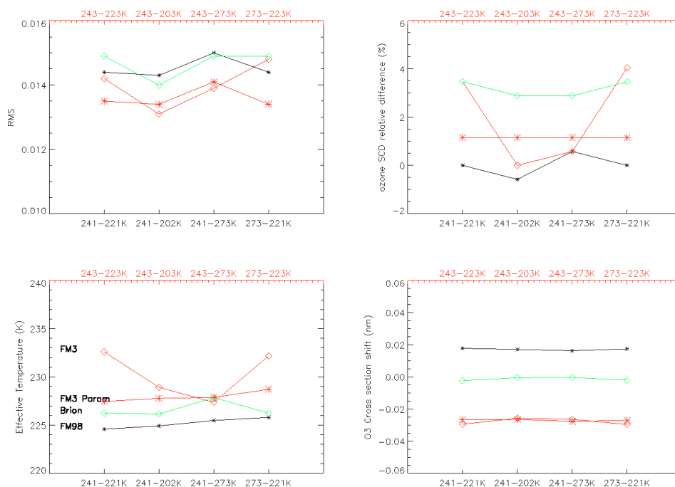
Figure 2 RMS fit residuals, O_3 slant column relative differences, effective temperatures and O_3 cross section wavelength shift from the DOAS ozone retrieval for pixel #8500 of GOME-2/MetOp-A Orbit 20392, using different combinations of O_3 absorption cross-section data sets.
