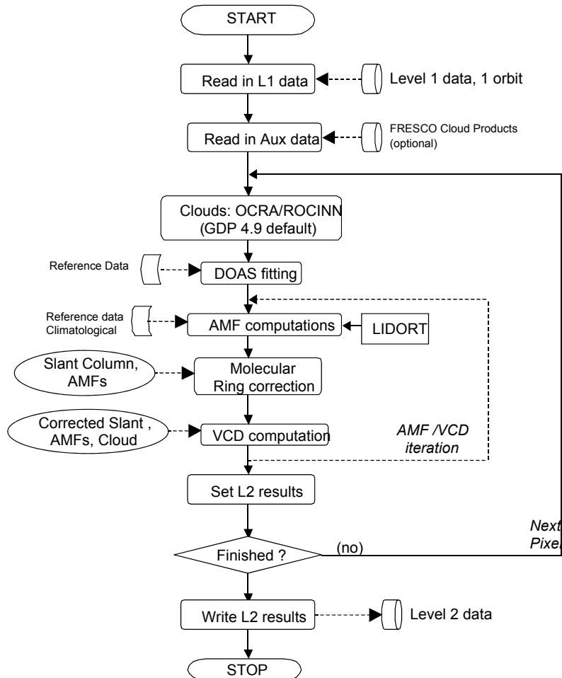
Figure 1 Flow diagram of the GDP trace gas column algorithm for GOME-2 (adapted from Van Roozendaal et al. (2006)). The molecular Ring correction and AMF/VCD iteration are specific ozone retrieval steps.
