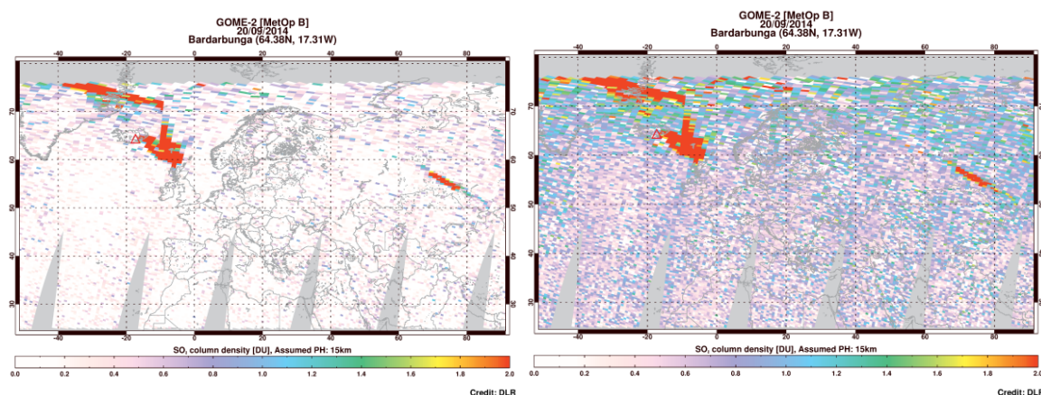
Figure 12 Effect of the background correction. The left image shows the background-corrected SO 2 vertical column from GOME-2/MetOp-B during the Bardarbunga eruption on 20 September 2014, whereas on the right image the correction is not applied.
