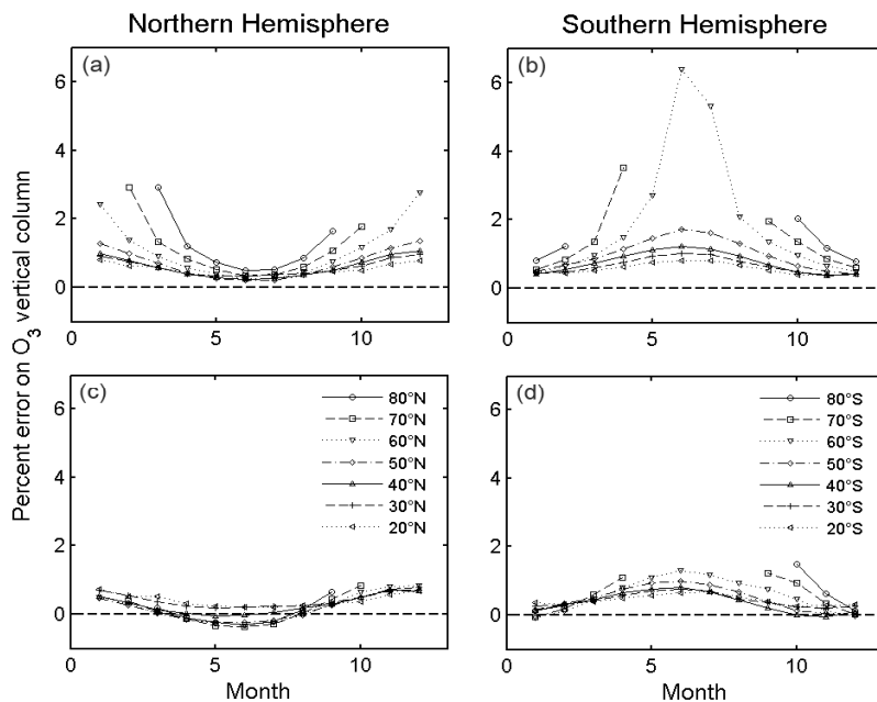
Figure 4 Impact on the total ozone accuracy of the choice of single wavelength for ozone AMF computations. Retrievals were made using synthetic radiance data based on the ozone profile climatology of Fortuin and Kelder (1998) (12 months, 7 latitude bands, both hemispheres). Panels (a) and (b): percentage error on total ozone columns for AMFs calculated at 325.0 nm. Panels (c) and (d): percentage error on total ozone with AMFs at 325.5 nm (from Van Roozendaal et al. (2006)).
