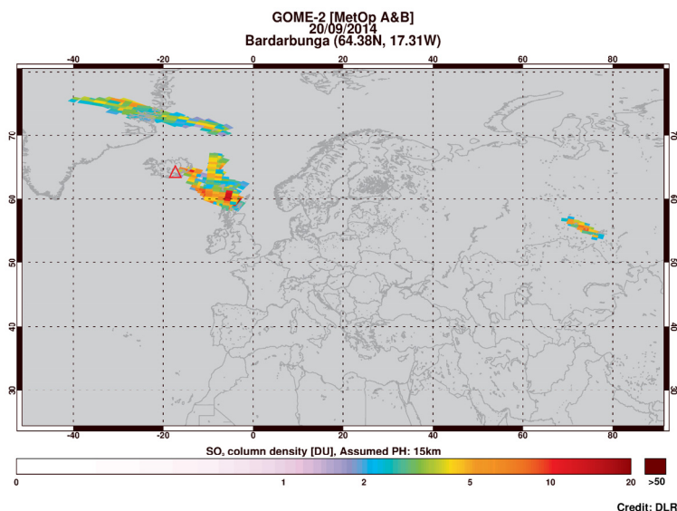
Figure 14 GOME-2 SO 2 measurement of the Bardarbunga volcanic eruption on 20 September 2014 from MetOp-A and -B. Only data flagged by the volcano activity detection algorithm is plotted, clearly showing the location of the SO 2 clouds.
