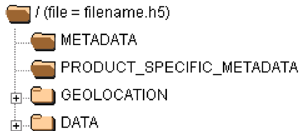
Figure 5.1: Structure of the HDF5 file.
