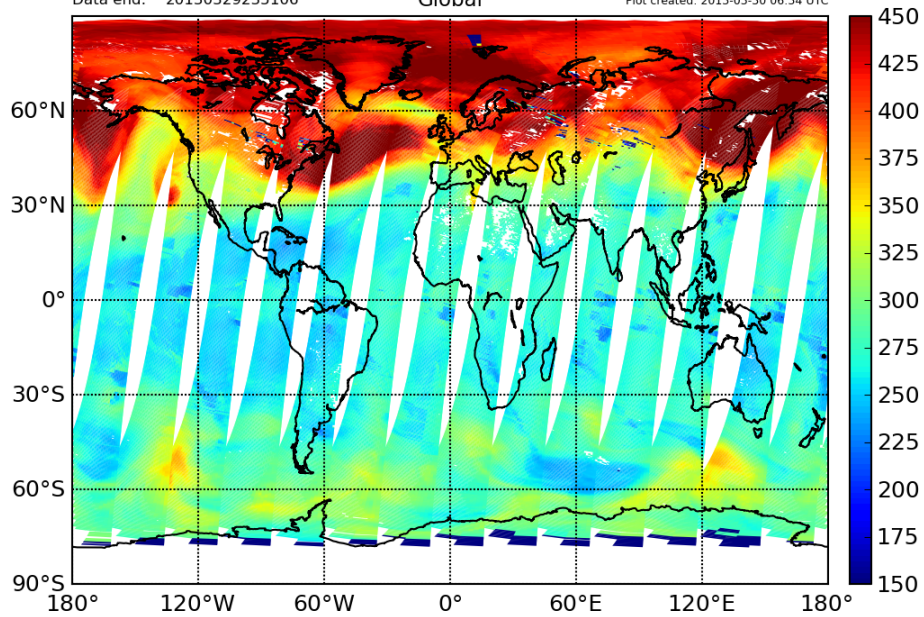
Figure 7.7: Integrated vertical ozone profile from GOME-2 on Metop-B, calculated as the sum of the retrieved profile on March 29th 2013.
