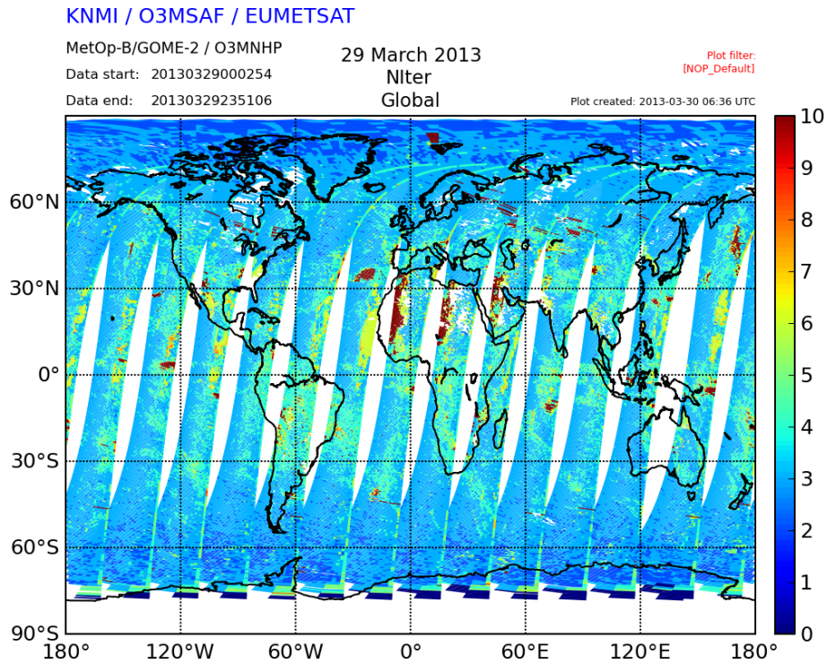
Figure 7.8: Number of iterations for each retrieval from GOME-2 on Metop-B on March 29th 2013. Brown pixels indicate non-converged profiles.
