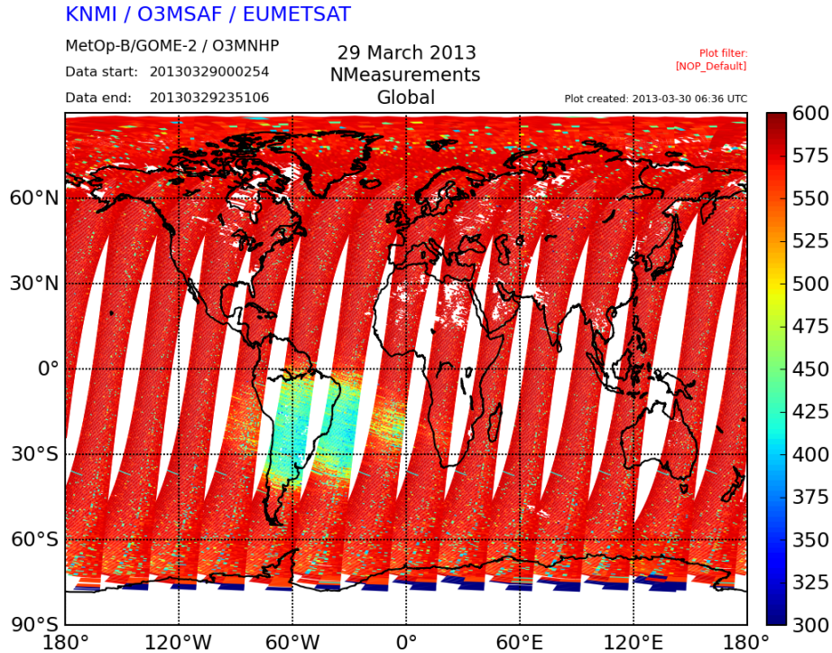
Figure 7.9: Number of spectral measurements of GOME-2 on Metop-B for each retrieved vertical ozone profile on March 29th 2013.
