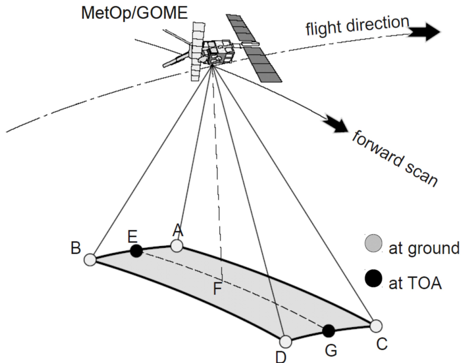
Figure 5: Ground Pixel Geometry
