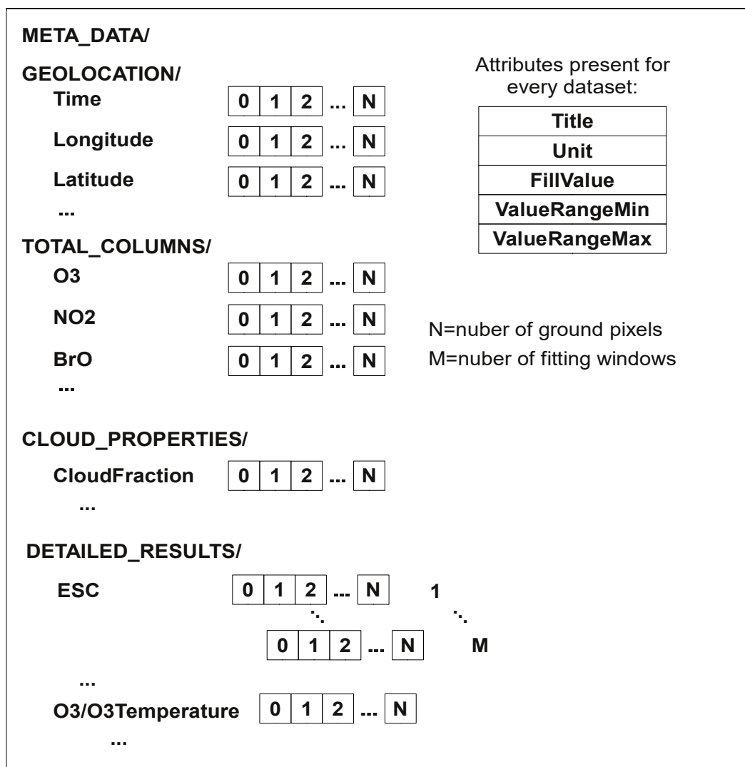
Figure 4: Organization of the GOME-2 total column products in the HDF5 structure
