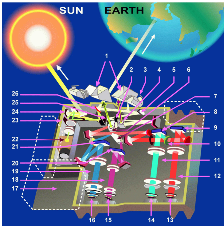
Figure 1: GOME optical layout (courtesy of ESA/ESTEC)
