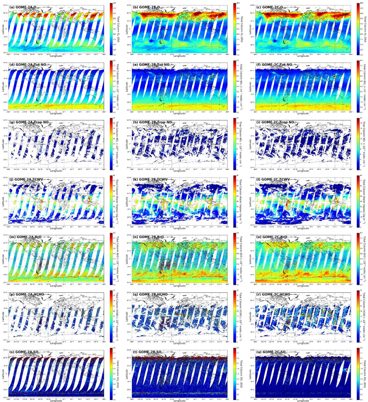
Figure 1. Daily level 3 product of GOME-2A (1 st column), GOME-2B (2 nd column), and GOME-2C (3 th column) for 15 January 2020. Total column O 3 (1 st row), total column NO 2 (2 nd row), tropospheric column NO 2 (3 th row), total column water vapour (4 th row), total column BrO (5 th row), total column HCHO (6 th row), and total column SO 2 (7 th row) are shown.
