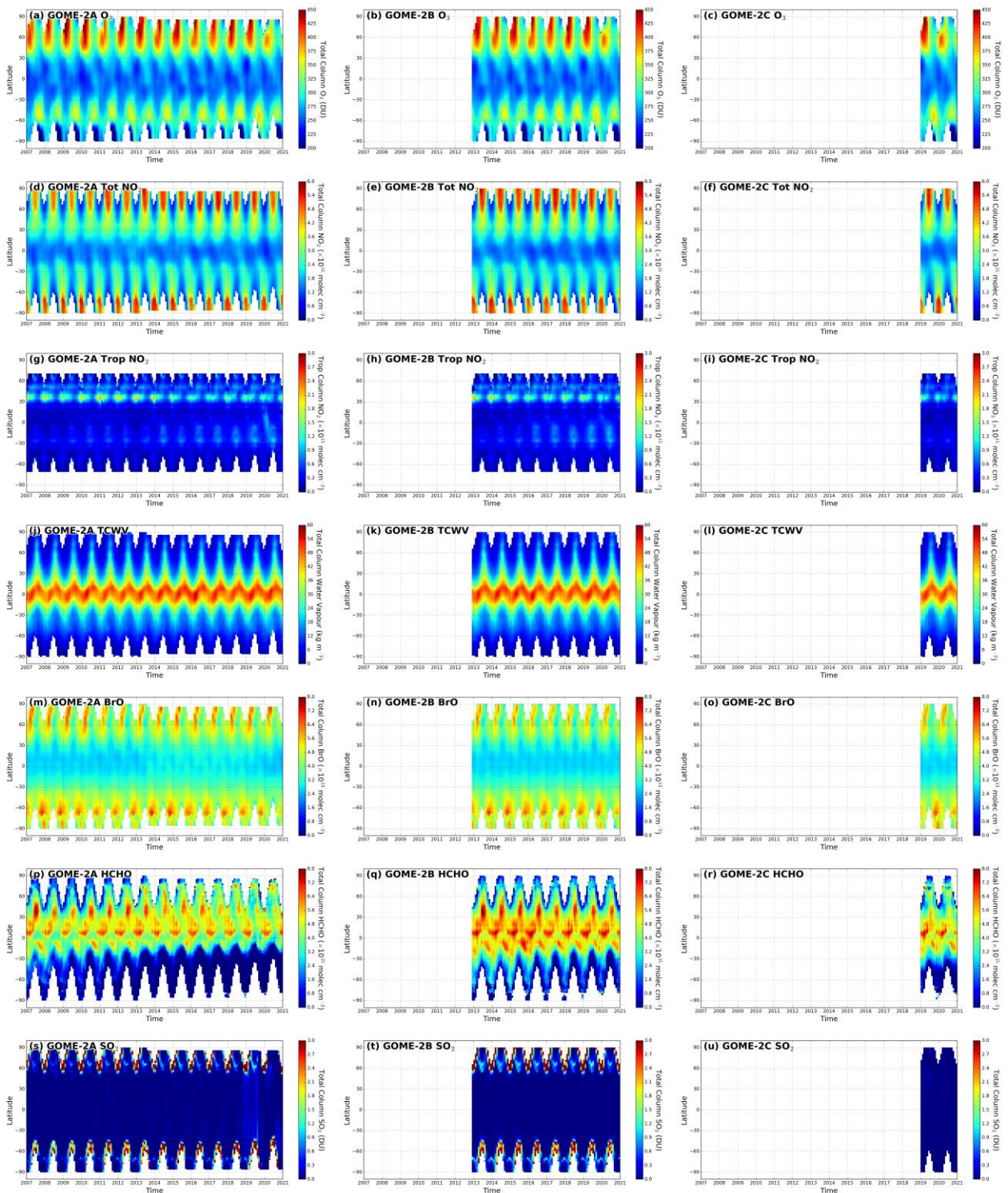
Figure 6. Monthly zonal average of total column O_3 (1 st row), total column NO_2 (2 nd row), tropospheric column NO_2 (3 rd row), total column water vapour (4 th row), total column BrO (5 th row), (total column HCHO (6 th row) and total column SO_2 (7 th row). Data from GOME-2A (1 st column from the left), GOME-2B (2 nd column from the left) and (3 rd column from the left) are shown.
