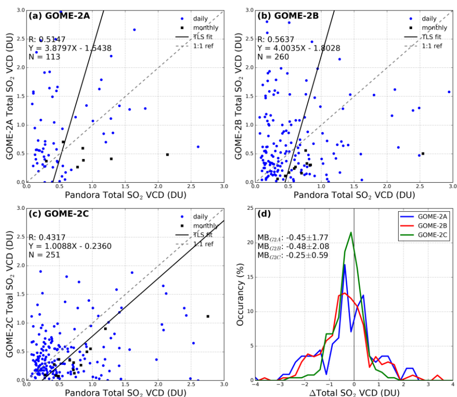
Figure 21. Comparison of daily and monthly total column SO 2 measured by Pandora instrument in Mexico City to (a) GOME-2A, (b) GOME-2B and (c) GOME-2C. Histograms of the difference of total column SO 2 between GOME-2 and Pandora observations are shown in (d).
