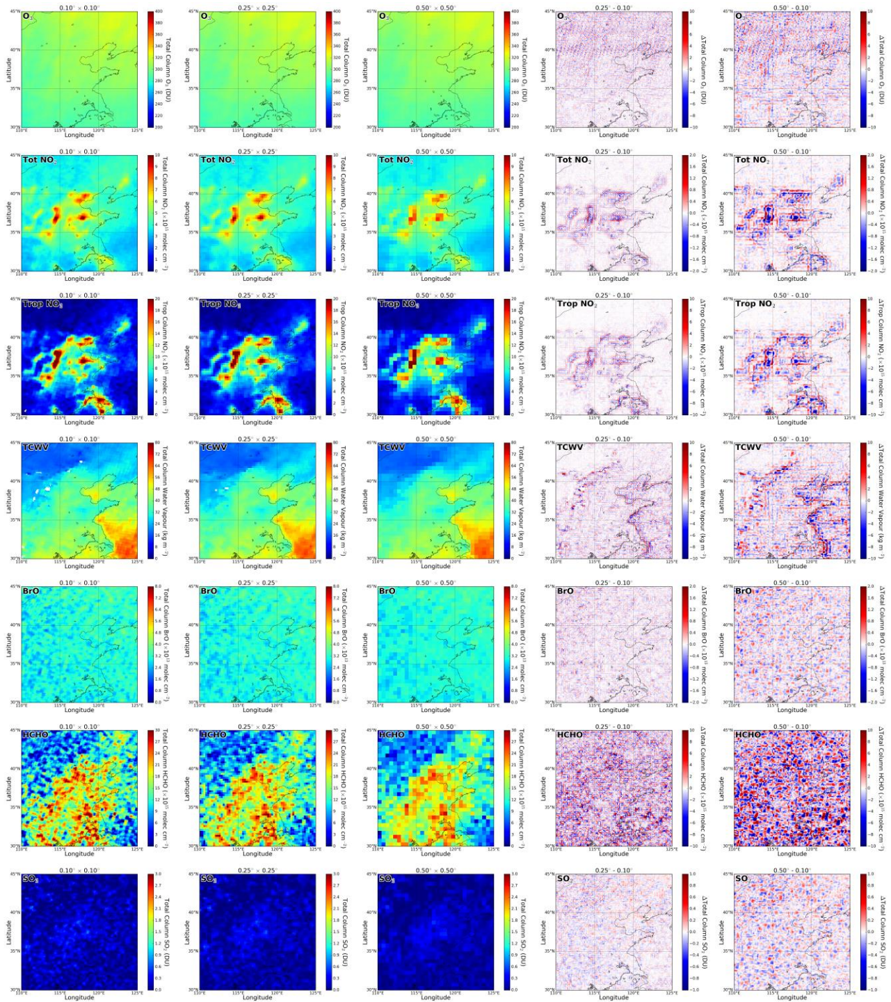
Figure 4. Monthly averaged GOME-2A observations of total column O 3 (1 st row), total column NO 2 (2 nd row), tropospheric column NO 2 (3 th row), total column water (4 th row), vapour total column BrO (5 th row), total column HCHO (6 th row), and total column SO 2 (7 th row) over North China in July 2014. Gridded data with 0.1° × 0.1° resolution (1 st column from the left), 0.25° × 0.25° resolution (2 nd column from the left), and 0.5° × 0.5° resolution (3 th column from the left) are shown. Differences between 0.1°, 0.25° and 0.5° are also shown for reference.
